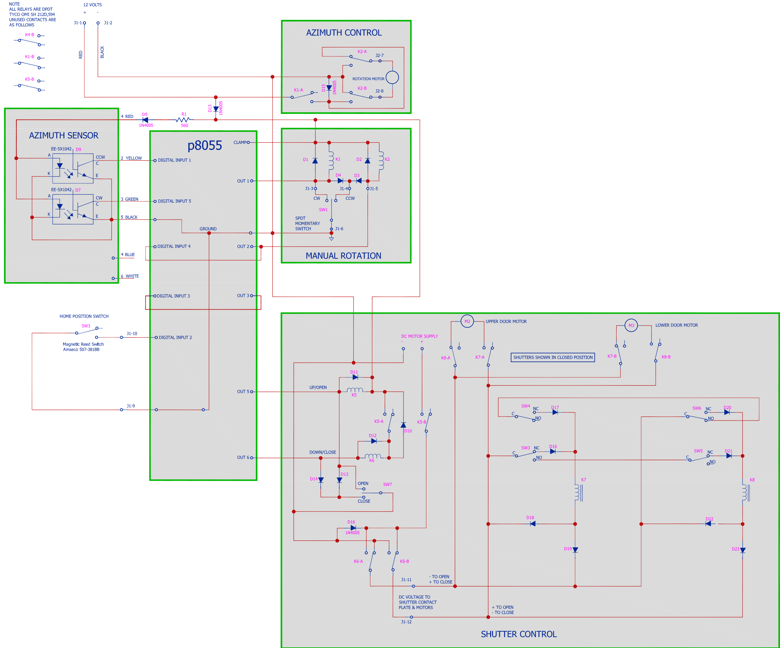
LESVEDOME SCHEMATIC WITHOUT DEAN MAN SWITCH OPTION
