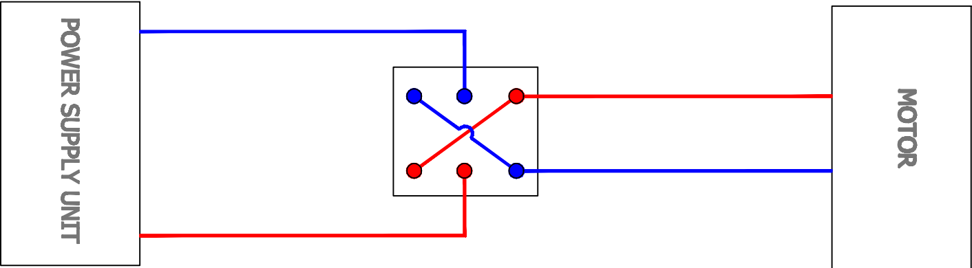
6 PIN MOMENTARY DPDT SWITCH
