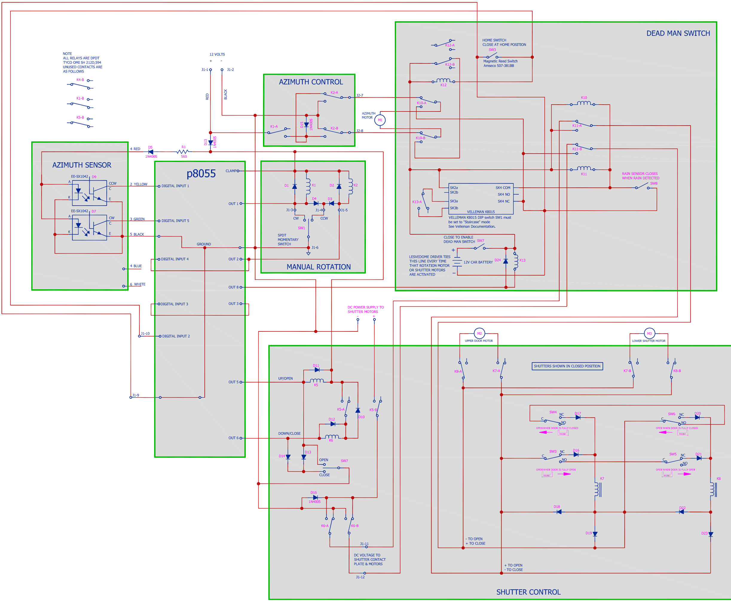
LESVEDOME SCHEMATIC WITH DEAN MAN SWITCH OPTION
